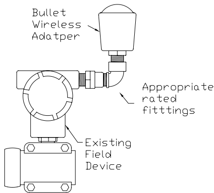
Figure 2: Typical Installation
